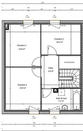
PLAN R+1
